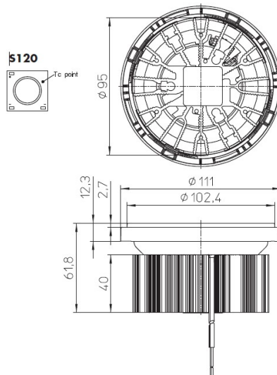
Heat sink 40 mm
